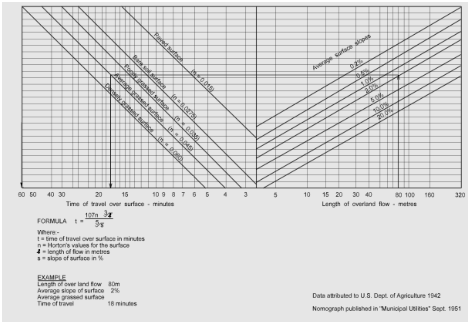
Figure 3: Overland flow graph
