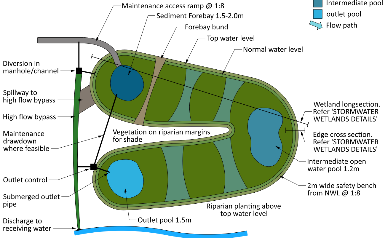
Schematic of Typical Offline Kidney Shaped (sinusoidal) Constructed Wetland
