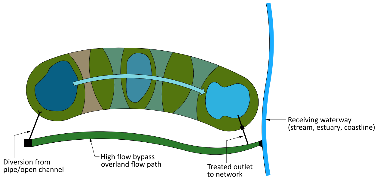
Schematic of Typical Zones in Offline Linear Constructed Wetland
