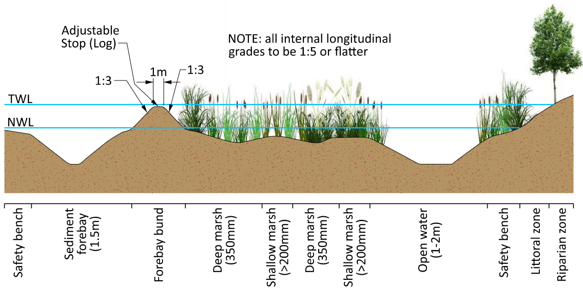
Wetland Bathymetry Diagram
