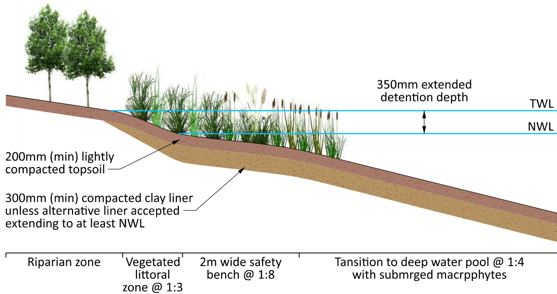
Typical Wetland Edge Detail Cross Section
