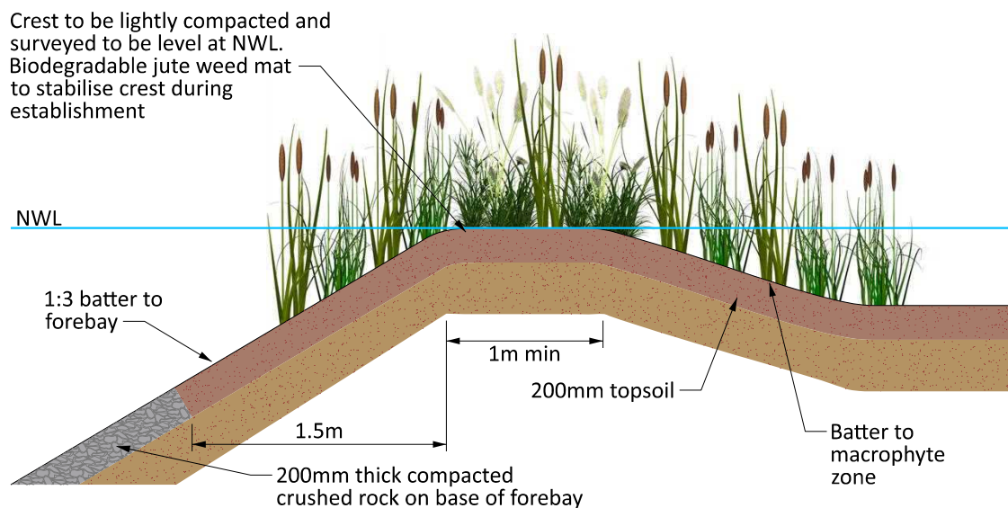
Typical Wetland Forebay Bund Cross Section
